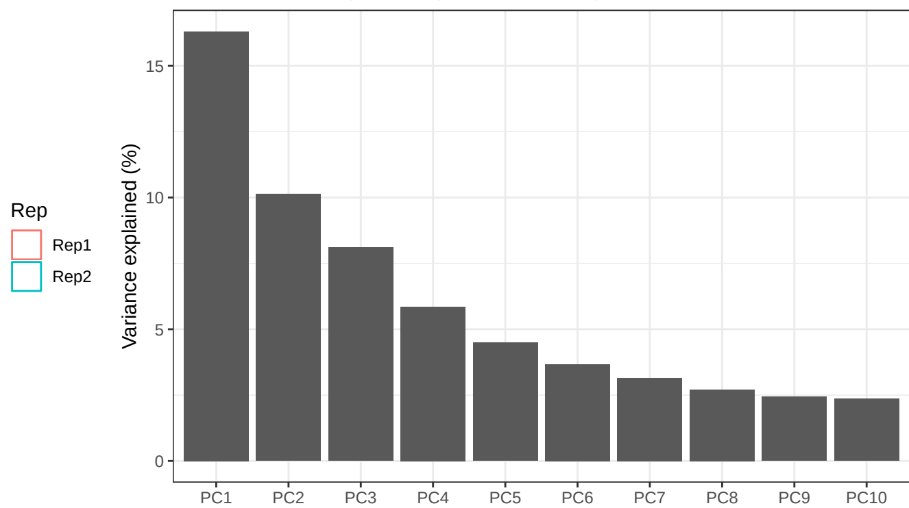
PCA variance explained (cleaned matrix)
